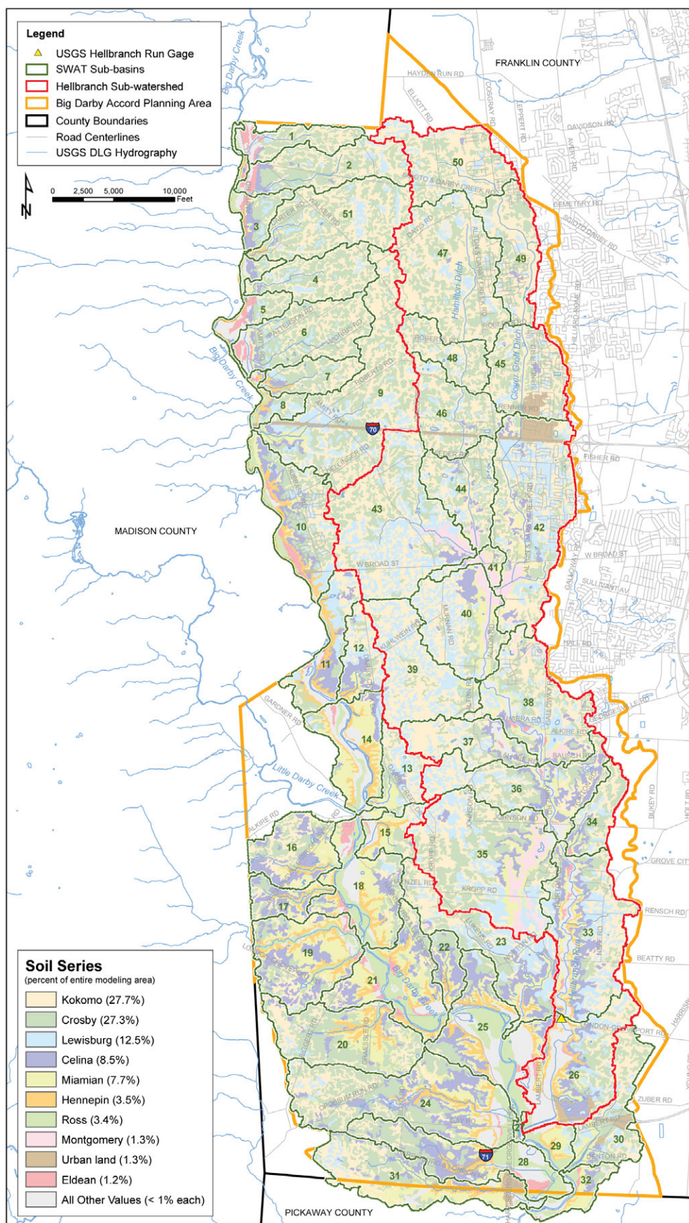
Figure 2: Soils Series (NRCS SSURGO Data)
