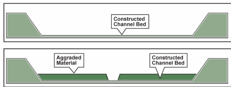
Figure 3.11 Over-wide Channel Design
